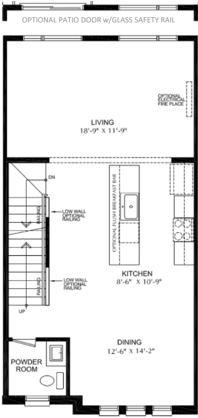
SECOND FLOOR 9' CEILING
