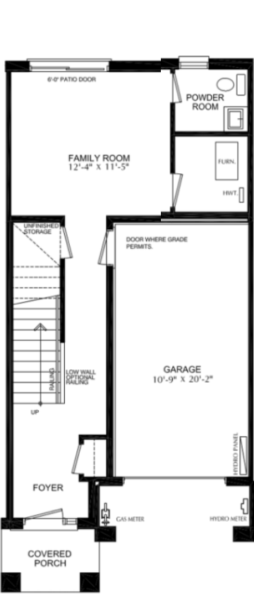
GROUND FLOOR 9' CEILING
